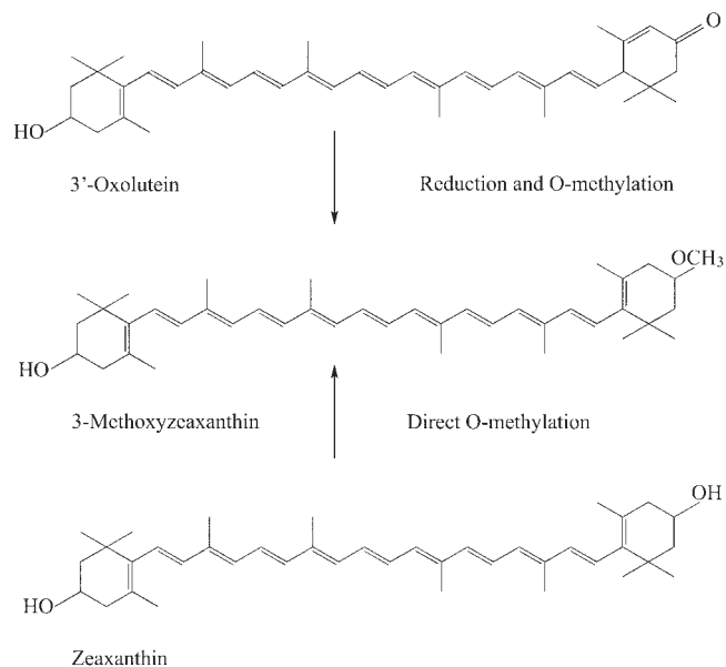
FIGURE 4. Structures and possible chemical conversions of zeaxanthin and 3'-oxolutein to 3-MZ.
