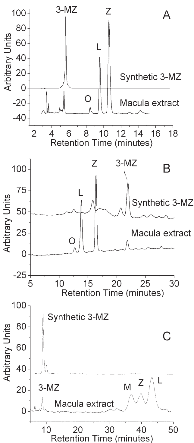
FIGURE 2. HPLC chromatograms of carotenoids extracted from the macula of a 73-year-old donor in comparison to synthetic 3-MZ. Analysis was performed on a silica nitrile column (A), a C30 column (B), and a chiral column (C). Major carotenoids found in the macula were (3 R ,3' R ,6' R )-lutein (L), (3 R ,3' R )-zeaxanthin (Z), (3 R ,3' S - meso )-zeaxanthin (M), 3-methoxyzeaxanthin (3-MZ), and 3'-oxolutein (O). Z and M co-eluted on columns A and B.
