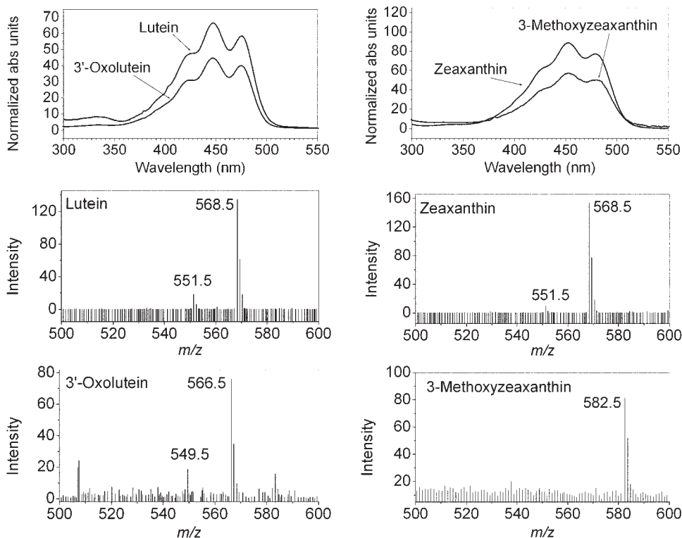
FIGURE 1. Absorption and mass spectra of lutein and zeaxanthin and their metabolites isolated and purified from human macula.
